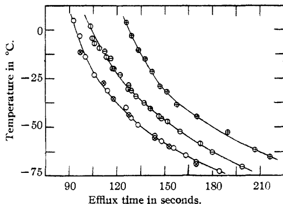
Fig. 2.—Time-temperature data: O, pure HF, exp. 1; ⊙, pure HF, exp. 2; ⊗, commercial HF, exp. 1; ◻, commercial HF, exp. 2; ⊕, alcohol-HF solution.
