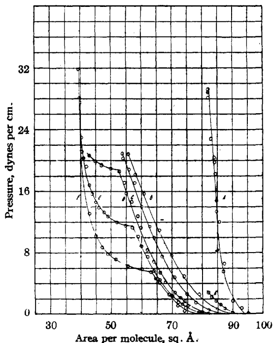
Fig. 1.—Monolayers of dilauryl maleate and dilauryl fumarate; A, fumarate, at 25°; pressure magnified 10 X; A', fumarate, at 25°; B, maleate, at 29°; C, maleate, at 25°; D, maleate, at 16°; E, maleate, at 9°; F, maleate, at 4°.
