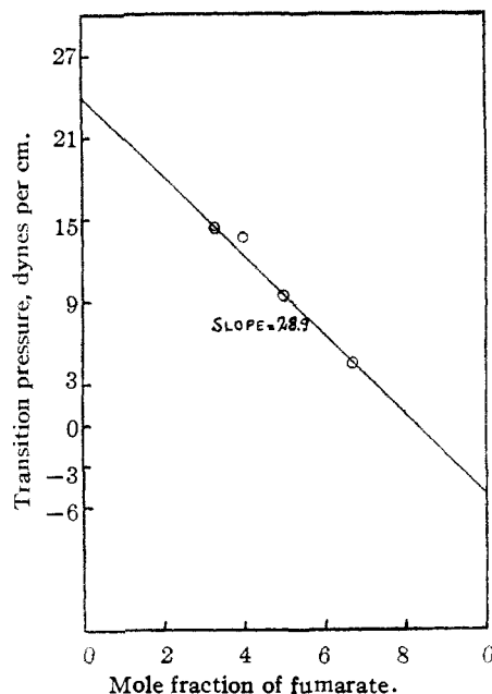
Fig. 4.—Raoult's law in monolayers.
