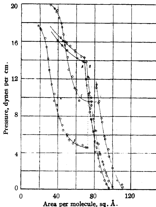
Fig. 2.—Mixed monolayers of dilauryl maleate and dilauryl fumarate: A, 2:1; B, 3:2; C, C', 1:1; D, D', 2:3.
