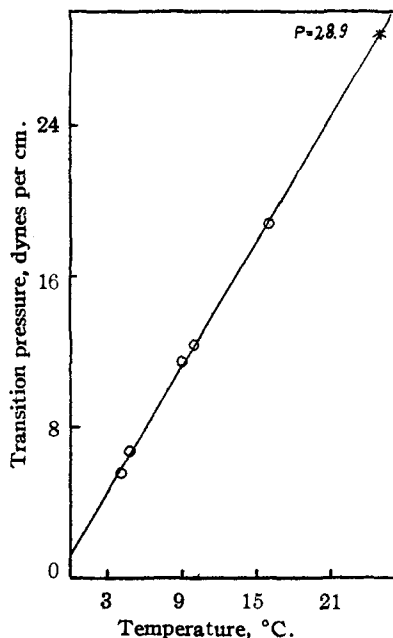
Fig. 3.—Condensation pressure and temperature in monolayers.
